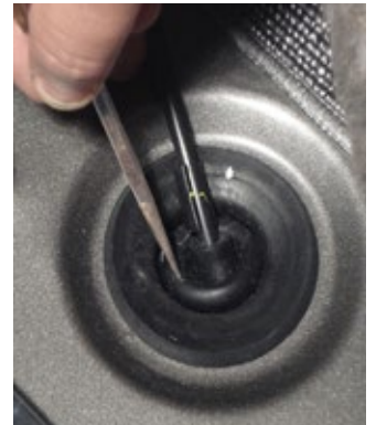
[Left] Factory grommet for wire routing. [Right] Using an awl, create access Passenger side factory grommet. Route wiring to Runner Platform Module [RPM12].
