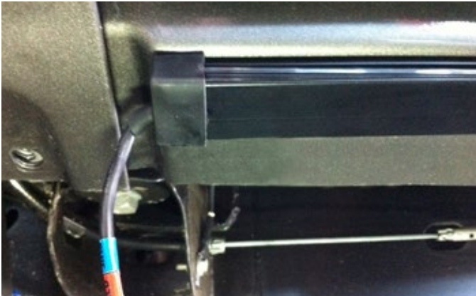
Detail view of correct placement of HG2 Runner assembly. Rear of HG2 Runner assembly aligns with body line as shown in previous photo.
