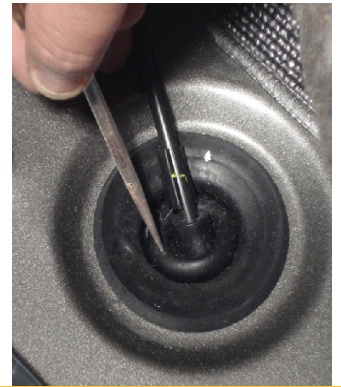
[Left] Factory grommet for wire routing. [Right] Using an awl, create access Passenger side factory grommet. Route wiring to Runner Platform Module [RPM12].
