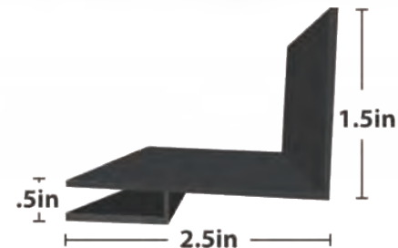
L - Bracket
